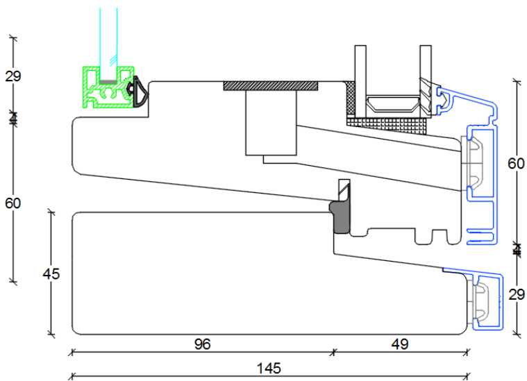
Lodret snit underkarm/ramme:
